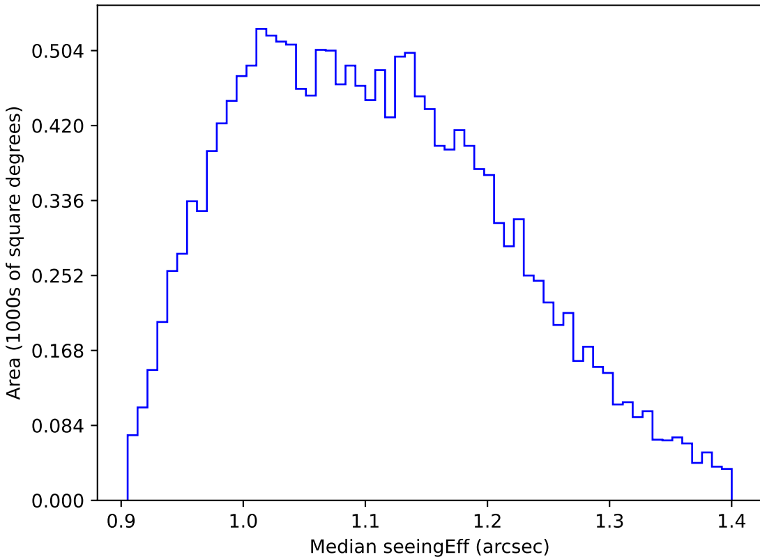
too_10_1v3.4_10yrs WFD g band: Median seeingEff
