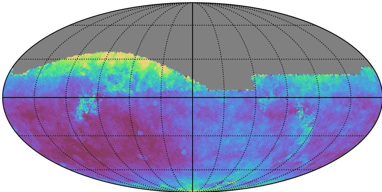
too_10_1v3.4_10yrs All sky z band: Median seeingEff
