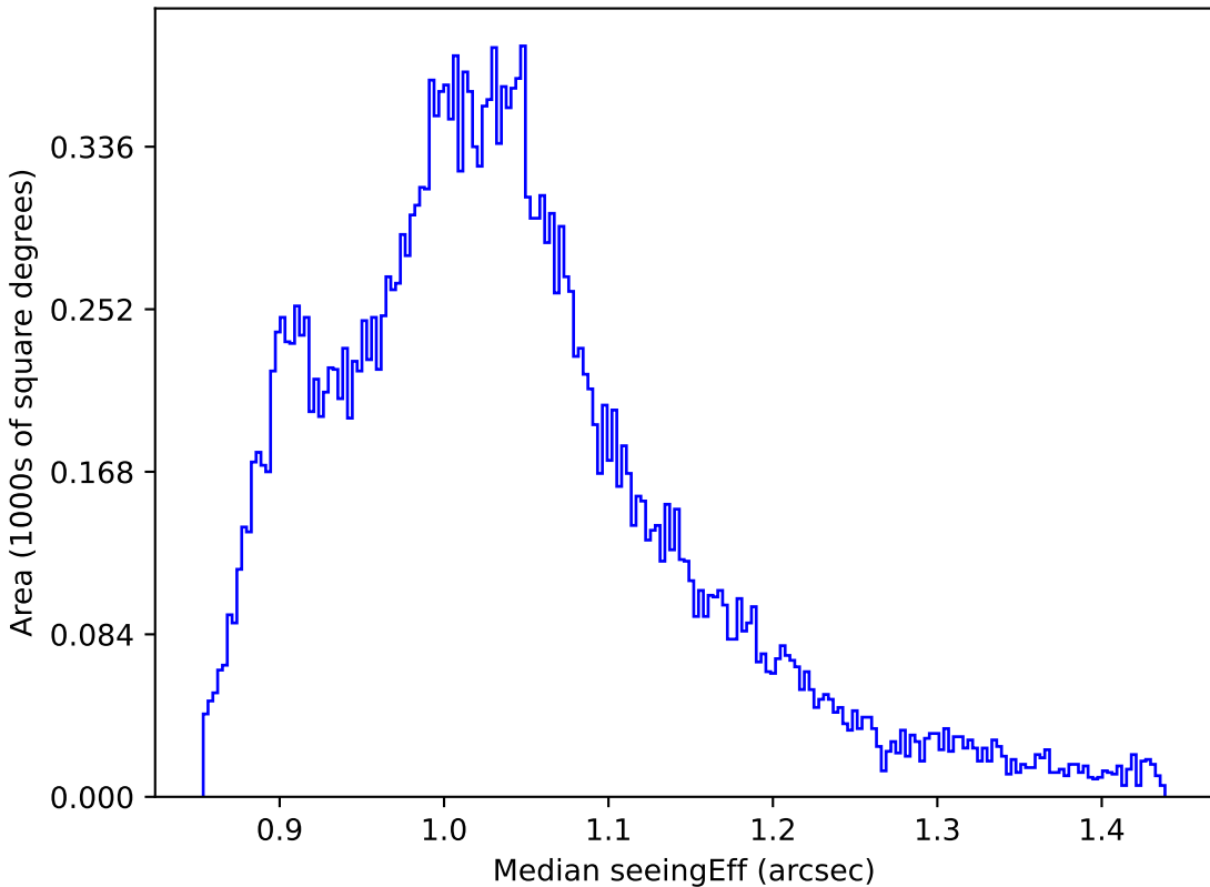
too_10_1v3.4_10yrs All sky z band: Median seeingEff
