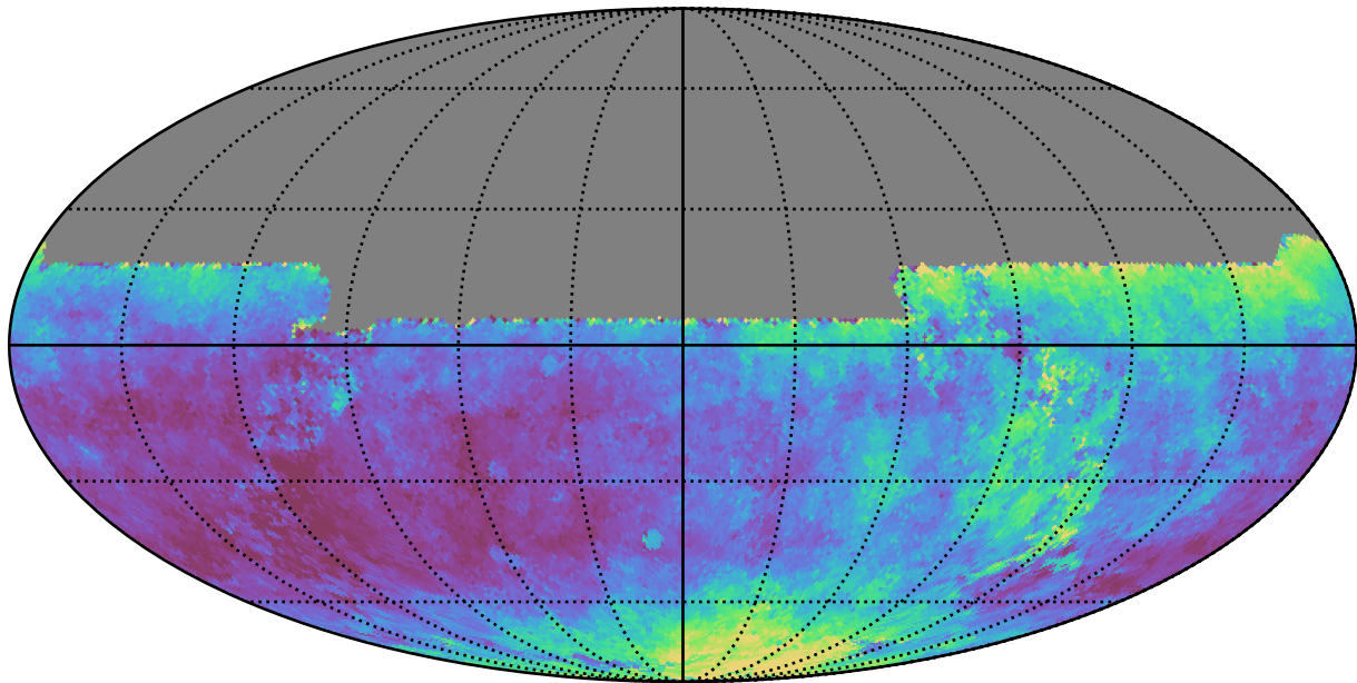
too_10_1v3.4_10yrs All sky y band: Median seeingEff
