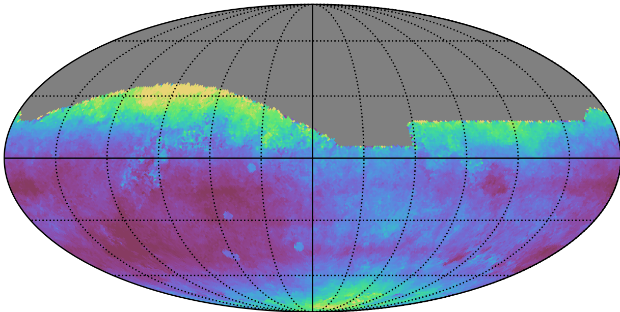
too_10_1v3.4_10yrs All sky r band: Median seeingEff
