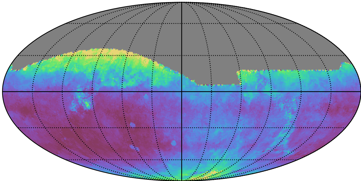
too_10_1v3.4_10yrs All sky i band: Median seeingEff
