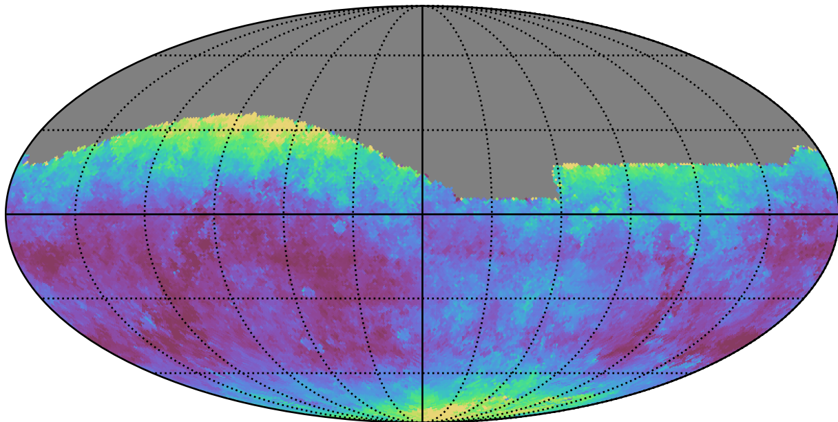
too_10_1v3.4_10yrs All sky g band: Median seeingEff
