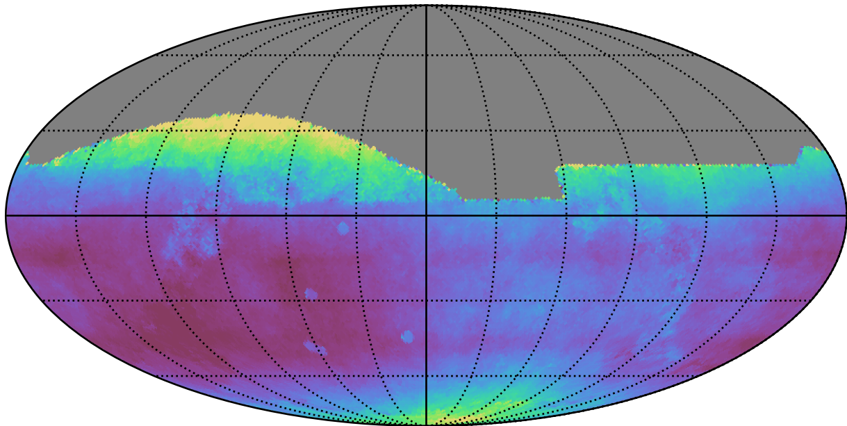
too_10_1v3.4_10yrs All sky all bands: Median seeingEff
