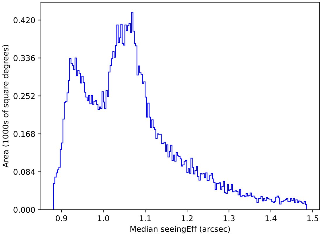
too_10_1v3.4_10yrs All sky all bands: Median seeingEff
