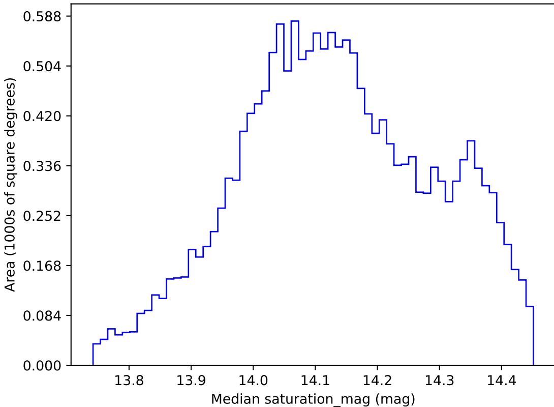
too_10_1v3.4_10yrs WFD z band: Median saturation_mag
