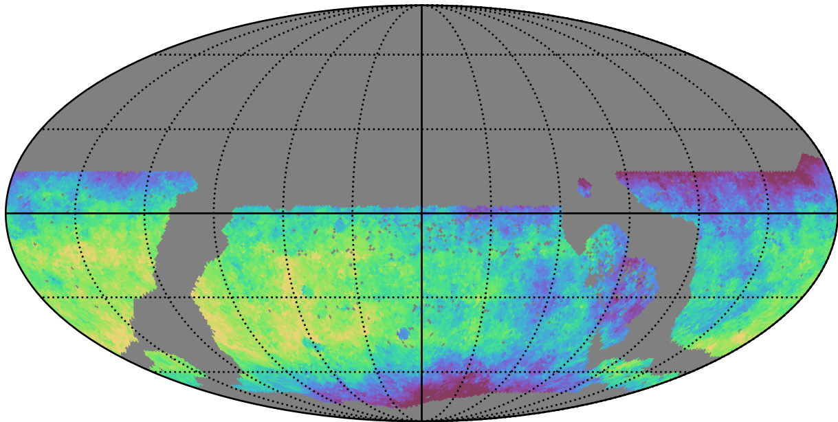
too_10_1v3.4_10yrs WFD y band: Median saturation_mag
