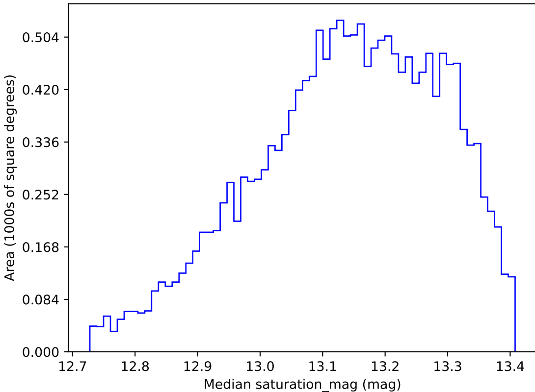
too_10_1v3.4_10yrs WFD y band: Median saturation_mag
