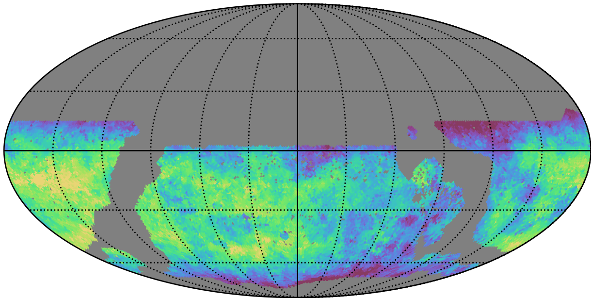
too_10_1v3.4_10yrs WFD u band: Median saturation_mag
