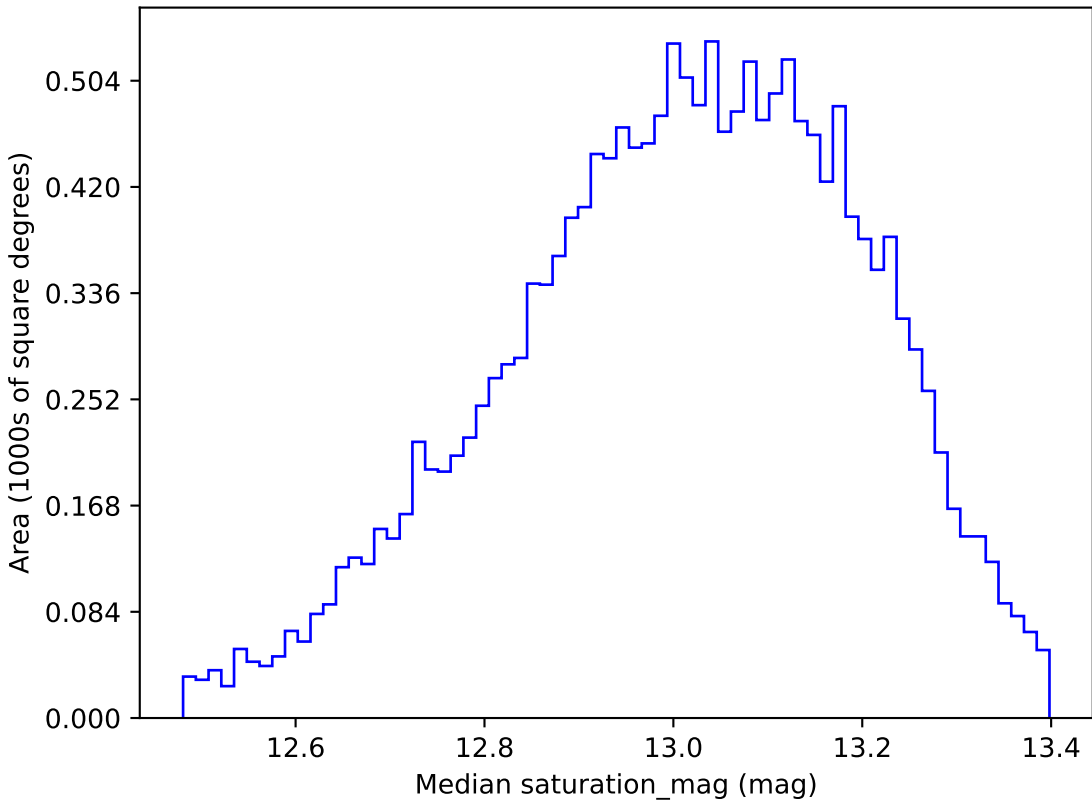
too_10_1v3.4_10yrs WFD u band: Median saturation_mag
