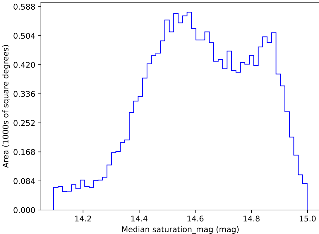
too_10_1v3.4_10yrs WFD r band: Median saturation_mag
