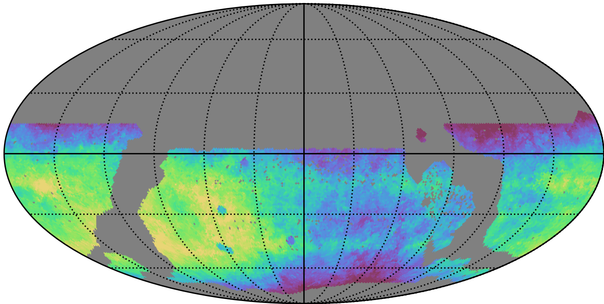
too_10_1v3.4_10yrs WFD i band: Median saturation_mag
