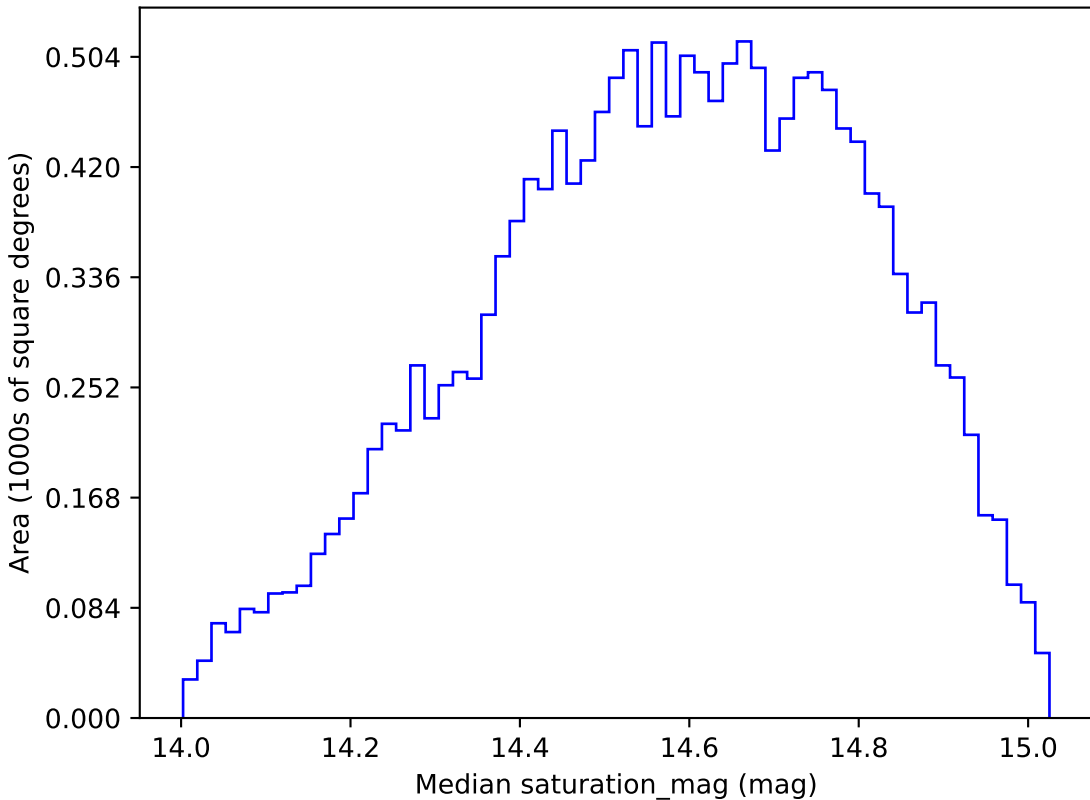
too_10_1v3.4_10yrs WFD g band: Median saturation_mag
