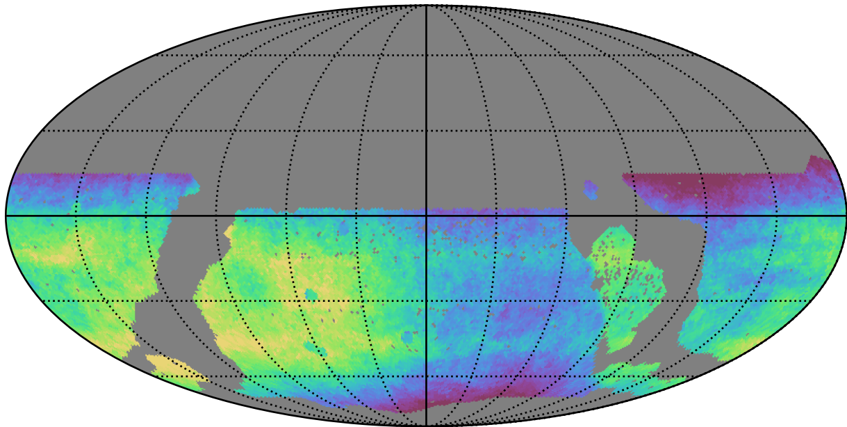
too_10_1v3.4_10yrs WFD all bands: Median saturation_mag
