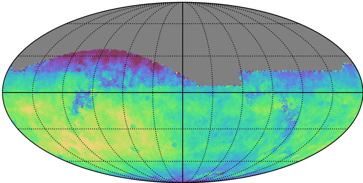
too_10_1v3.4_10yrs All sky z band: Median saturation_mag
