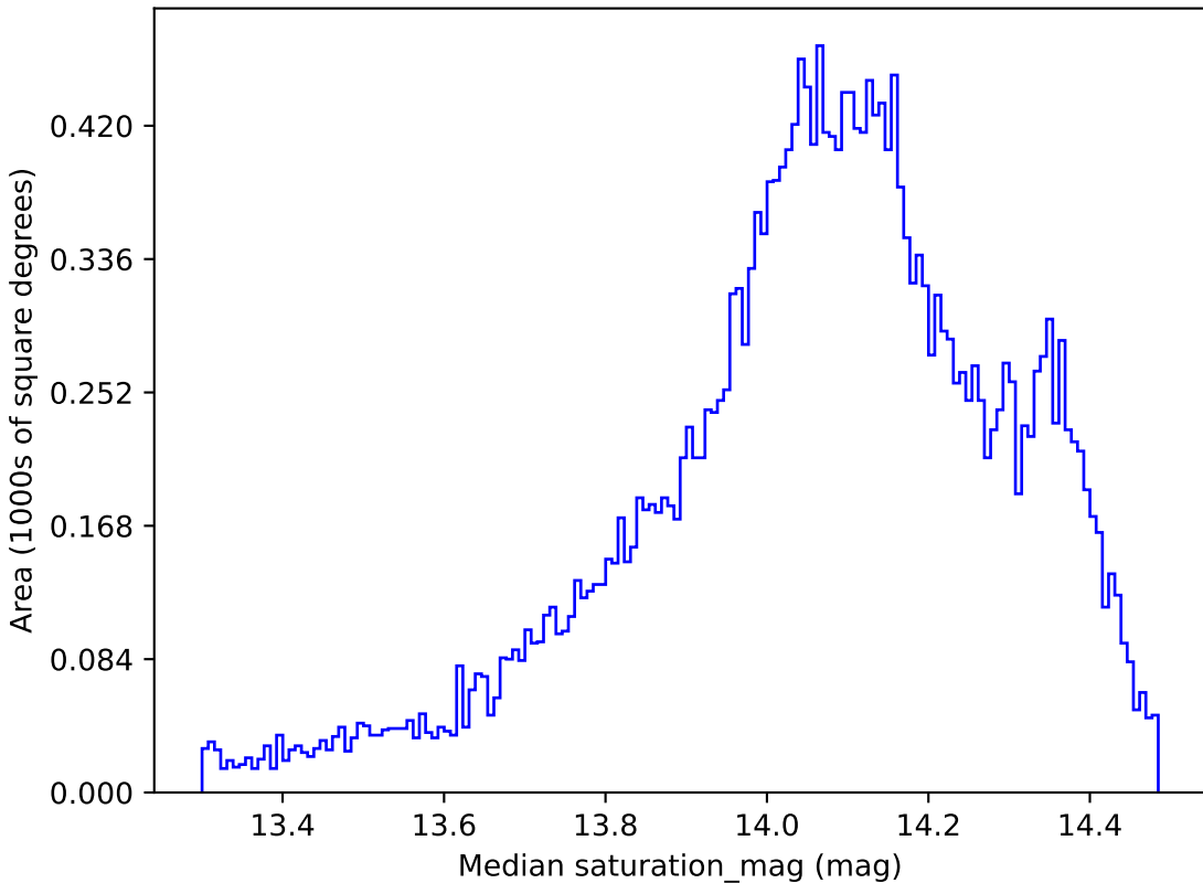
too_10_1v3.4_10yrs All sky z band: Median saturation_mag
