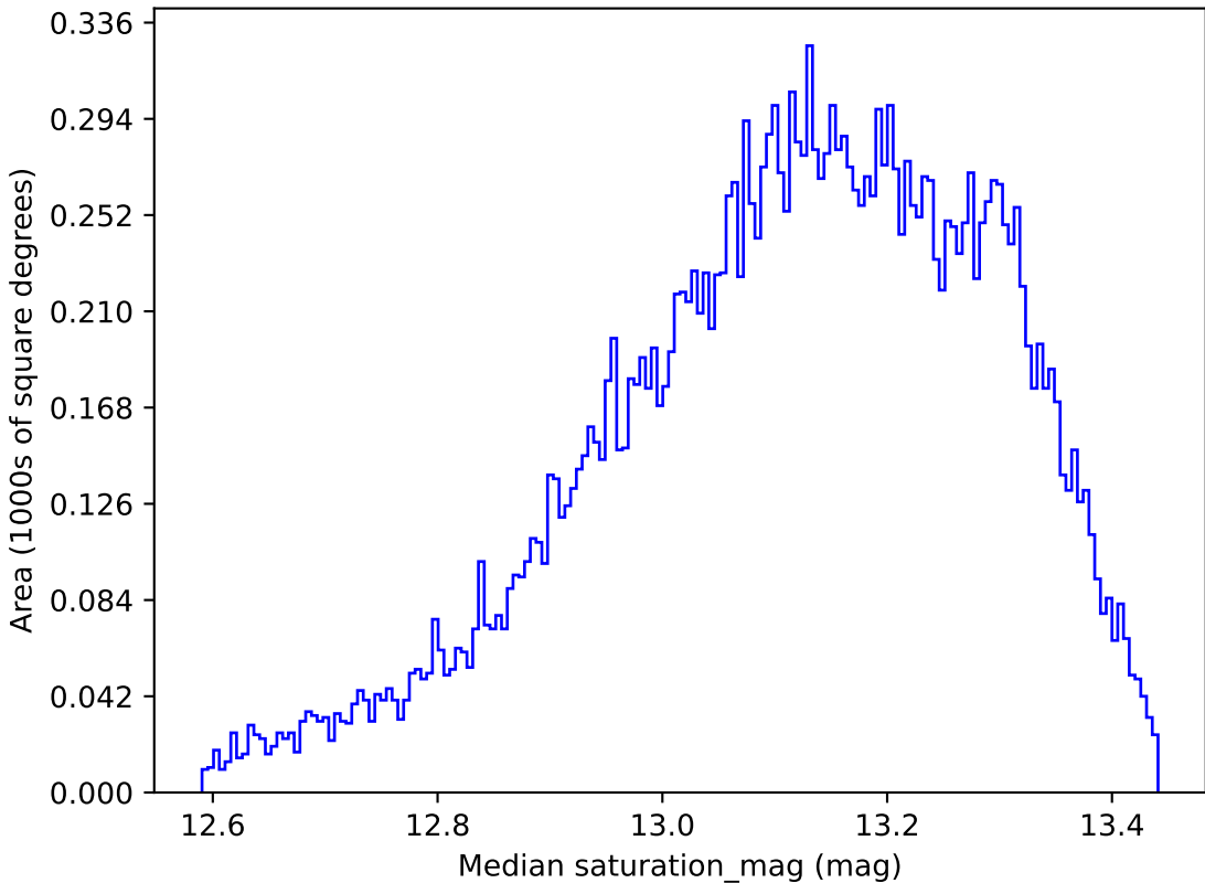
too_10_1v3.4_10yrs All sky y band: Median saturation_mag
