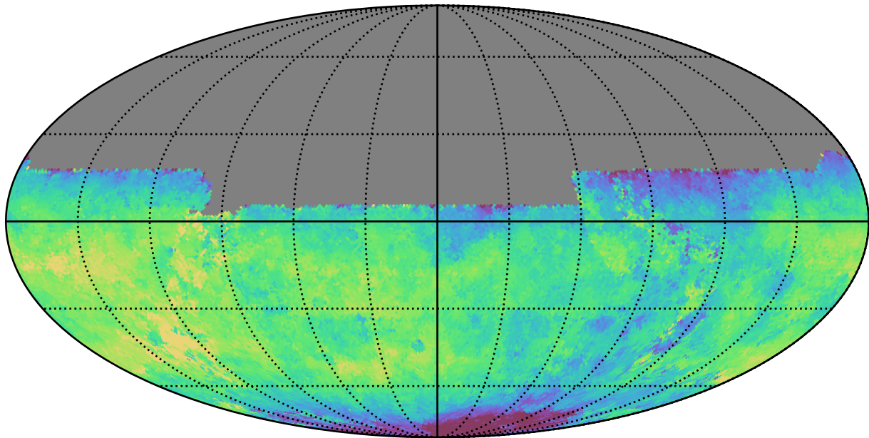
too_10_1v3.4_10yrs All sky u band: Median saturation_mag
