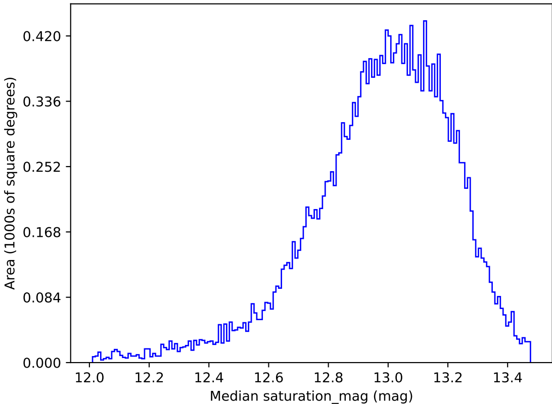
too_10_1v3.4_10yrs All sky u band: Median saturation_mag
