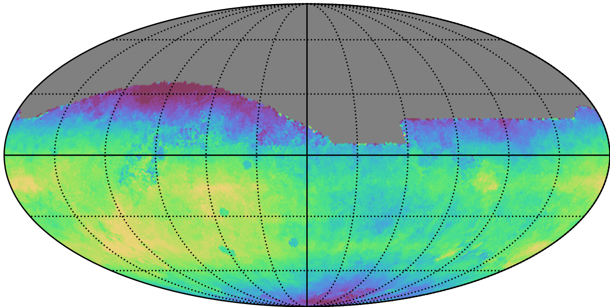
too_10_1v3.4_10yrs All sky r band: Median saturation_mag
