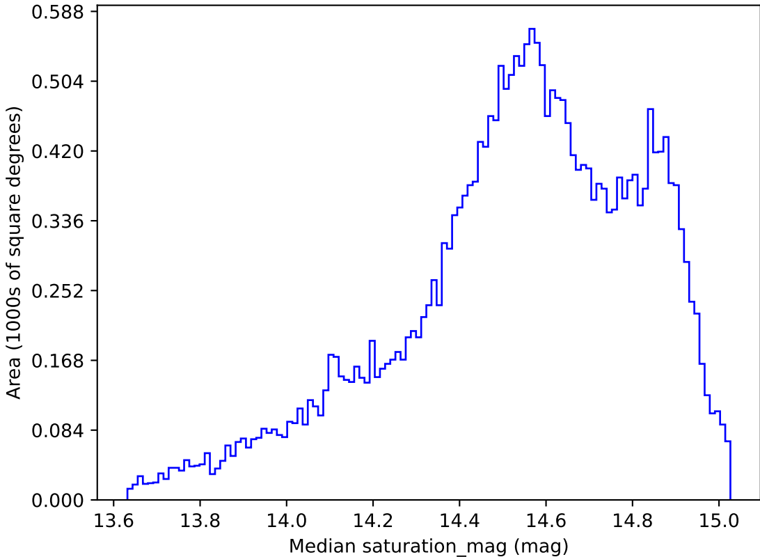
too_10_1v3.4_10yrs All sky r band: Median saturation_mag
