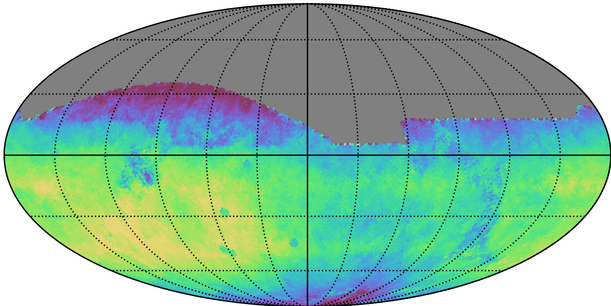
too_10_1v3.4_10yrs All sky i band: Median saturation_mag
