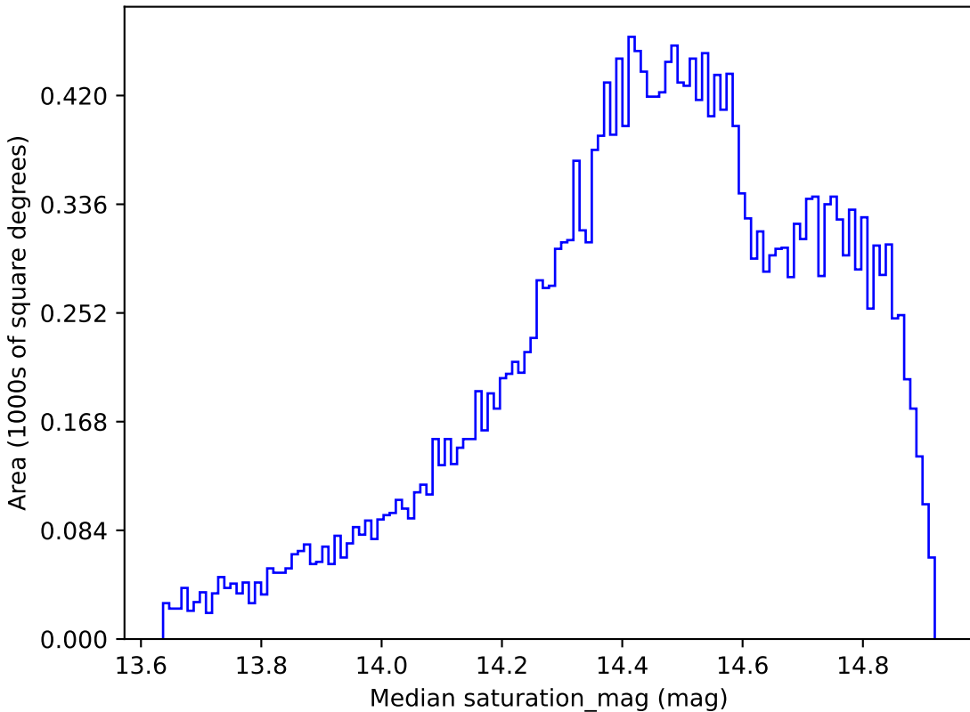
too_10_1v3.4_10yrs All sky i band: Median saturation_mag
