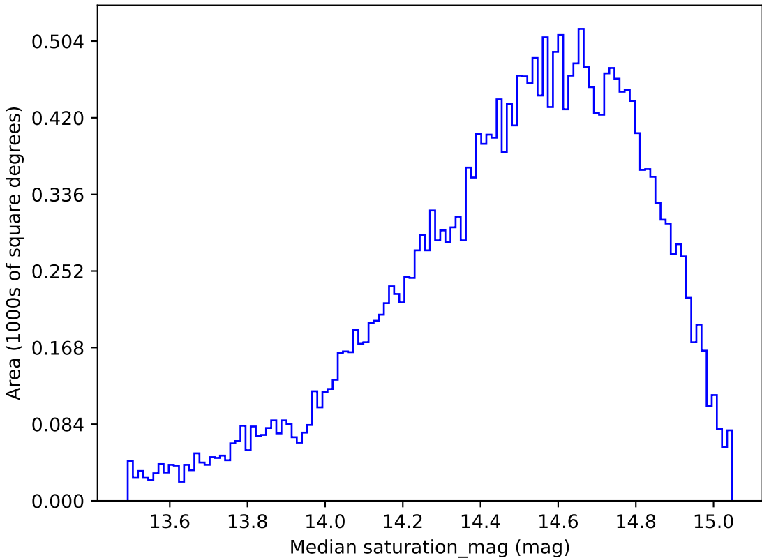
too_10_1v3.4_10yrs All sky g band: Median saturation_mag
