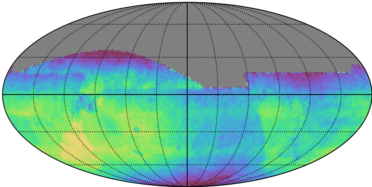
too_10_1v3.4_10yrs All sky all bands: Median saturation_mag
