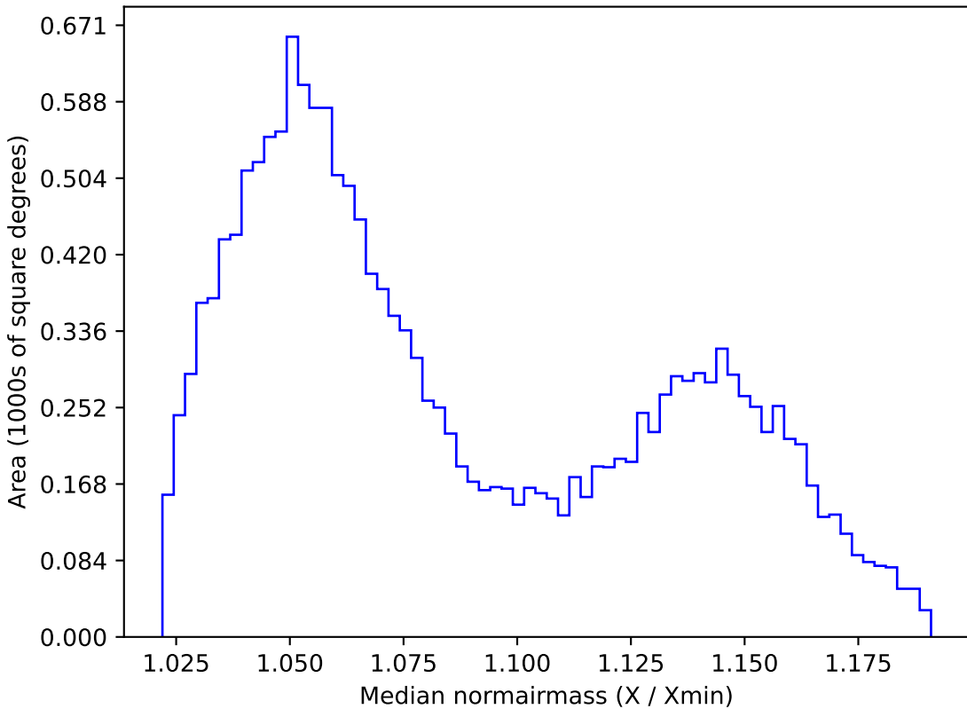
too_10_1v3.4_10yrs WFD z band: Median normairmass
