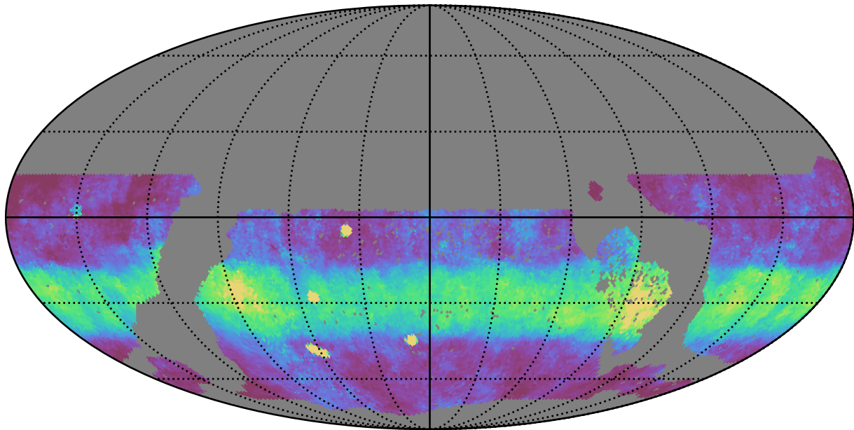
too_10_1v3.4_10yrs WFD y band: Median normairmass
