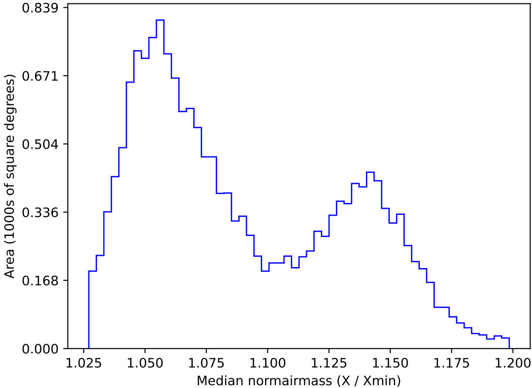
too_10_1v3.4_10yrs WFD y band: Median normairmass
