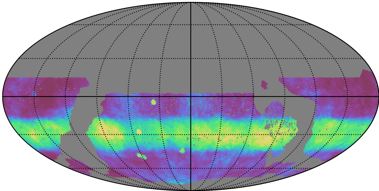
too_10_1v3.4_10yrs WFD i band: Median normairmass
