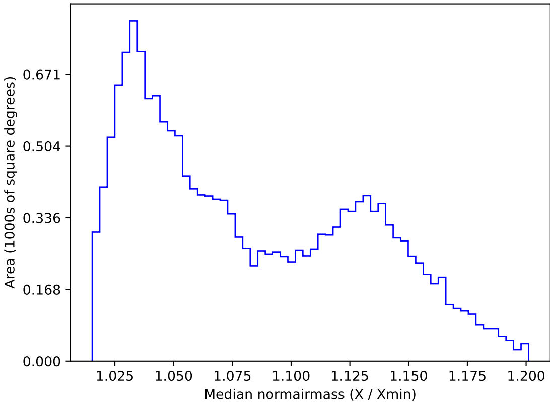
too_10_1v3.4_10yrs WFD g band: Median normairmass
