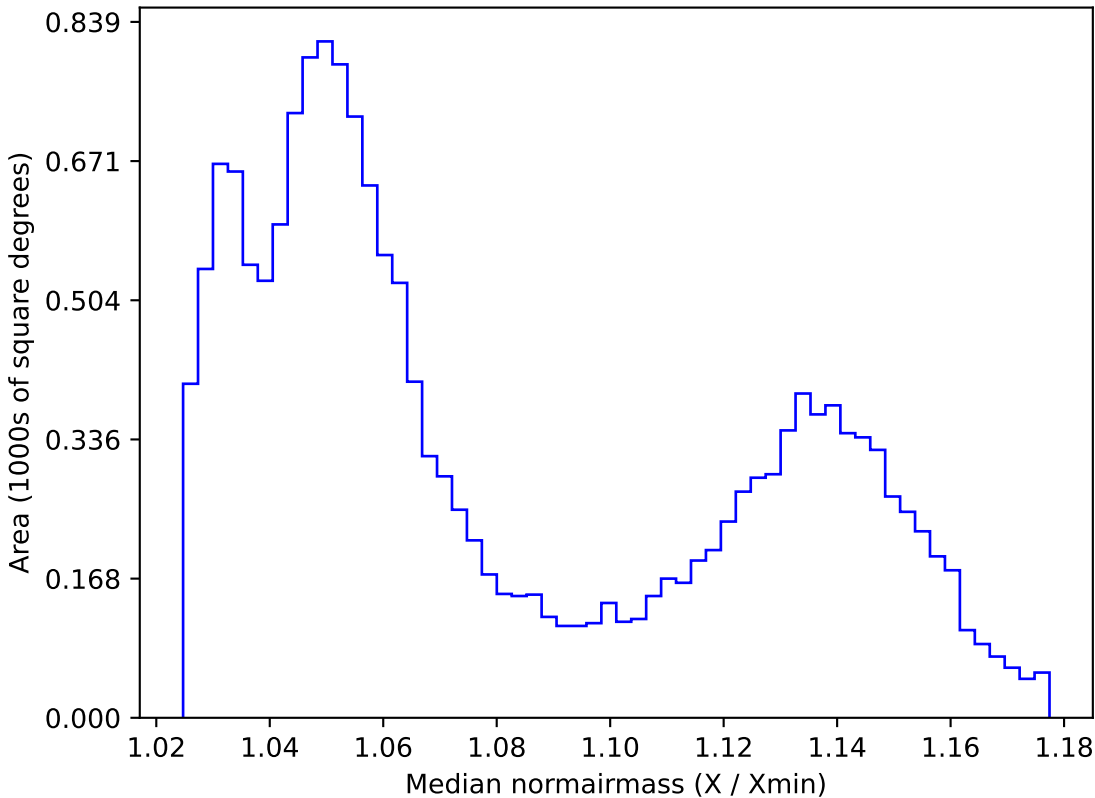
too_10_1v3.4_10yrs WFD all bands: Median normairmass
