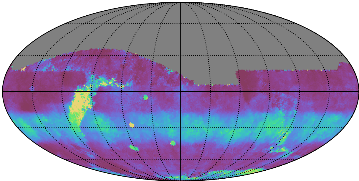
too_10_1v3.4_10yrs All sky z band: Median normairmass
