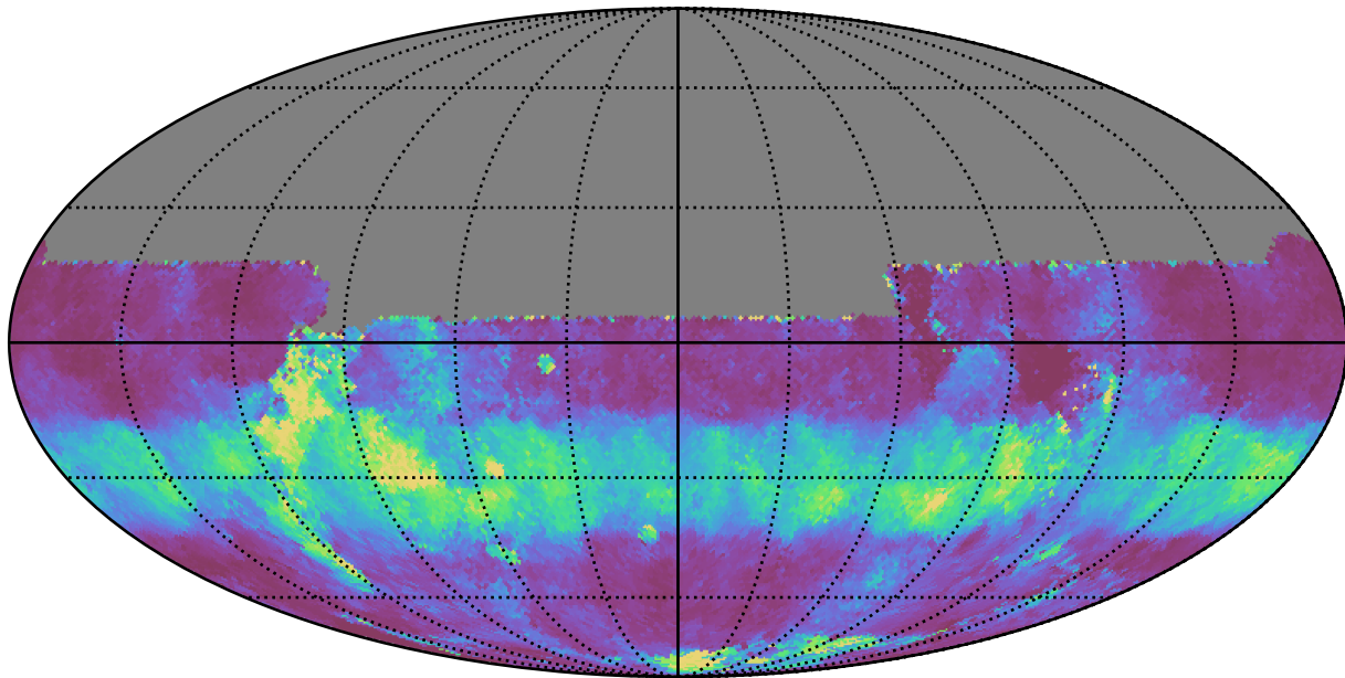
too_10_1v3.4_10yrs All sky u band: Median normairmass
