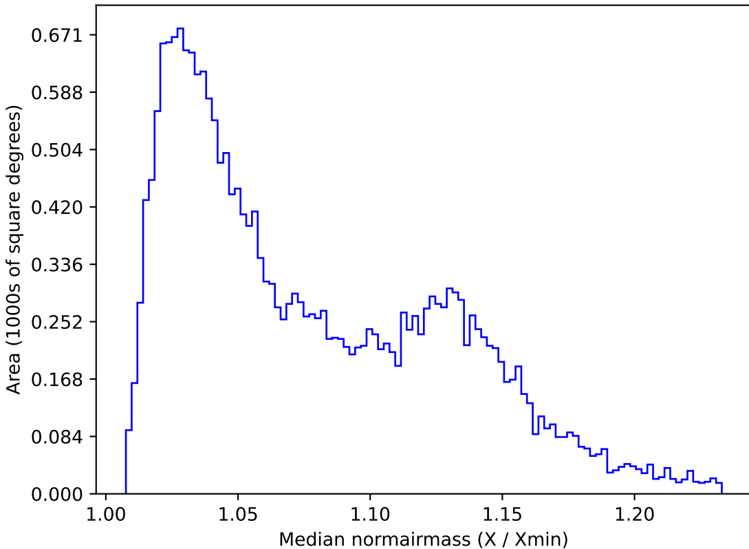
too_10_1v3.4_10yrs All sky u band: Median normairmass
