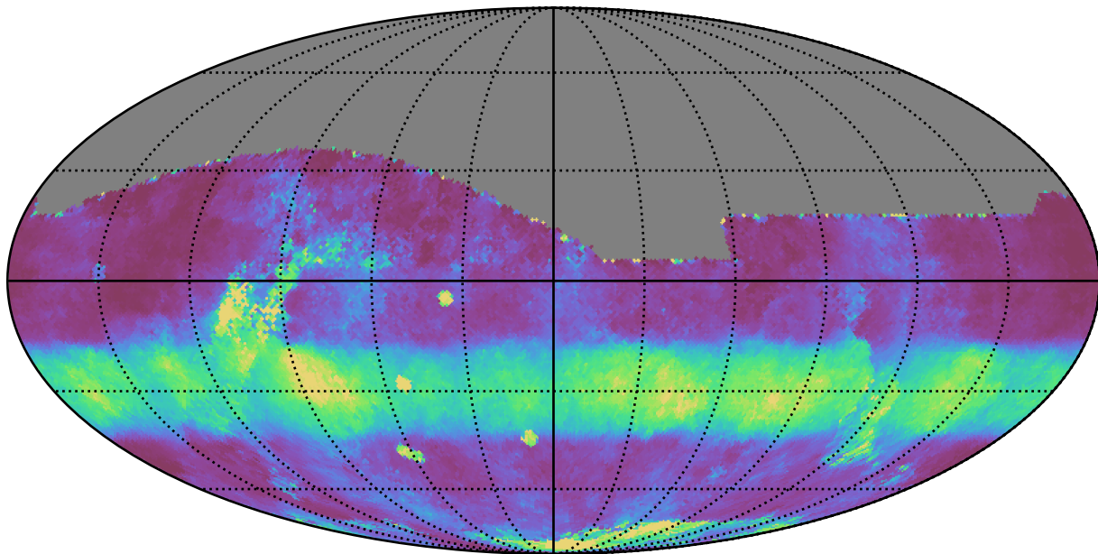
too_10_1v3.4_10yrs All sky r band: Median normairmass
