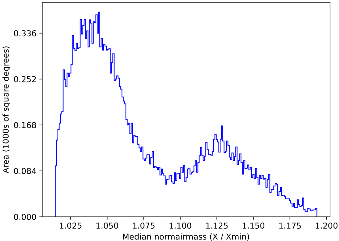
too_10_1v3.4_10yrs All sky r band: Median normairmass
