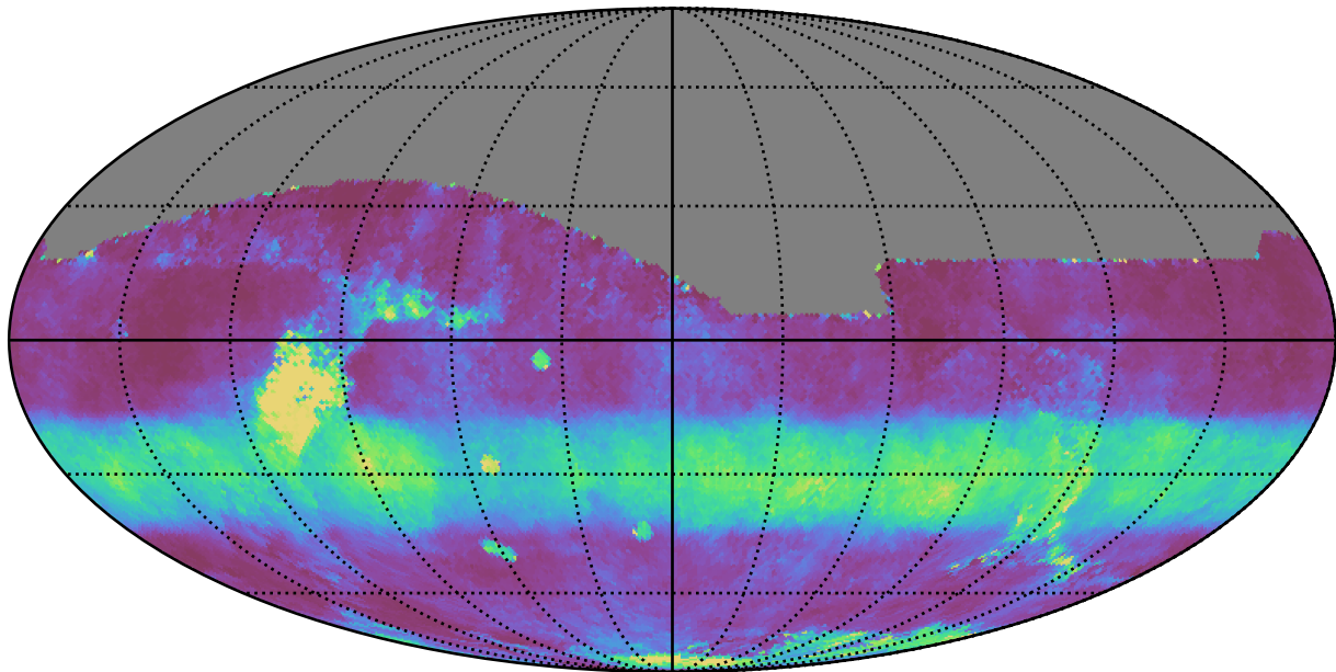
too_10_1v3.4_10yrs All sky i band: Median normairmass
