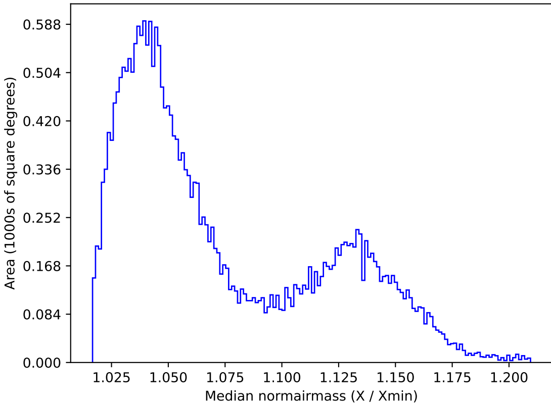
too_10_1v3.4_10yrs All sky i band: Median normairmass
