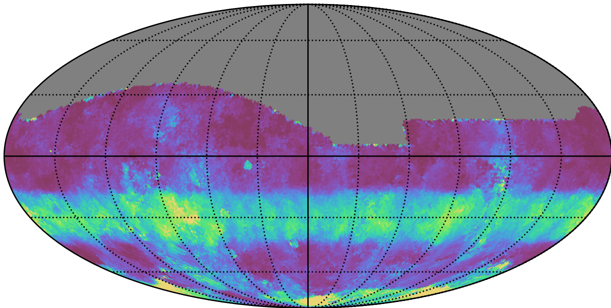
too_10_1v3.4_10yrs All sky g band: Median normairmass
