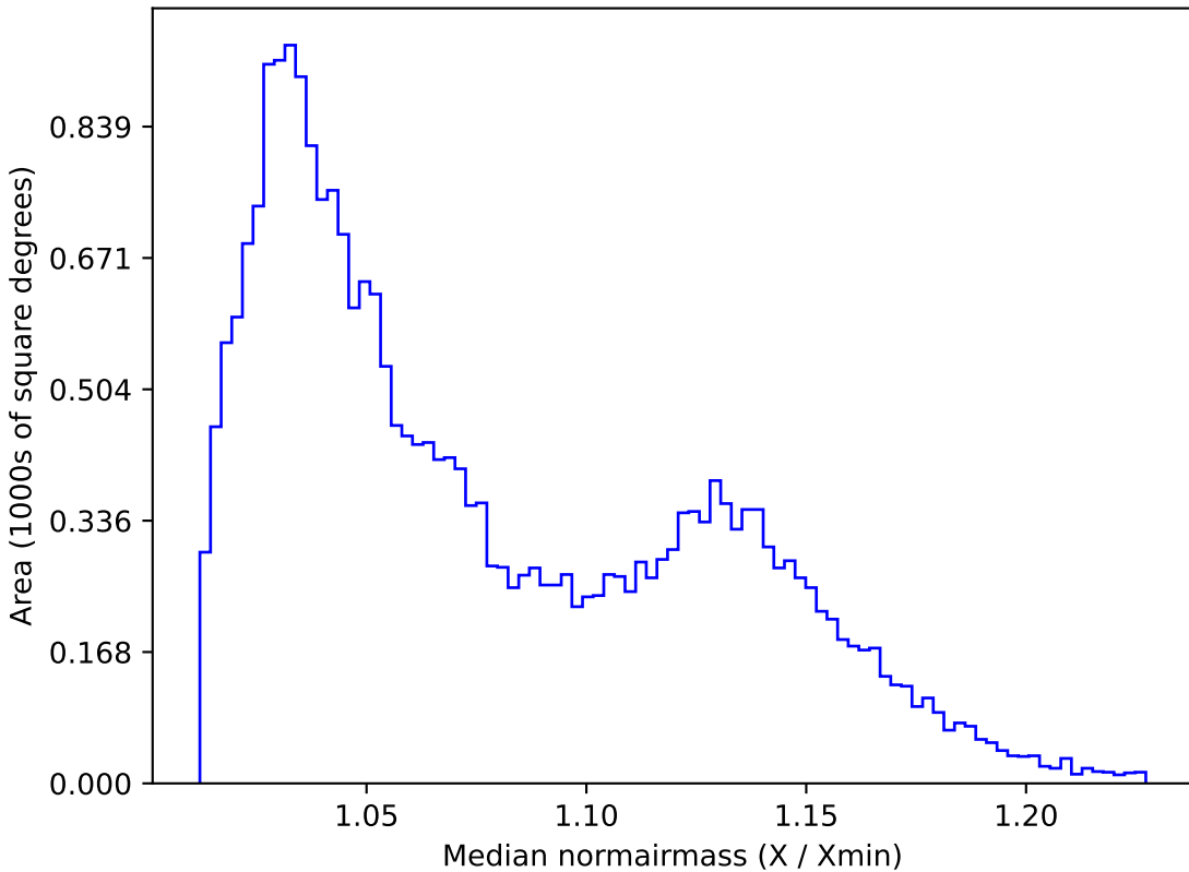
too_10_1v3.4_10yrs All sky g band: Median normairmass
