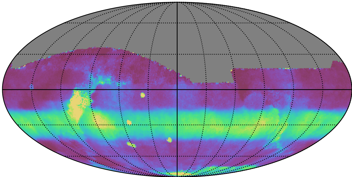
too_10_1v3.4_10yrs All sky all bands: Median normairmass
