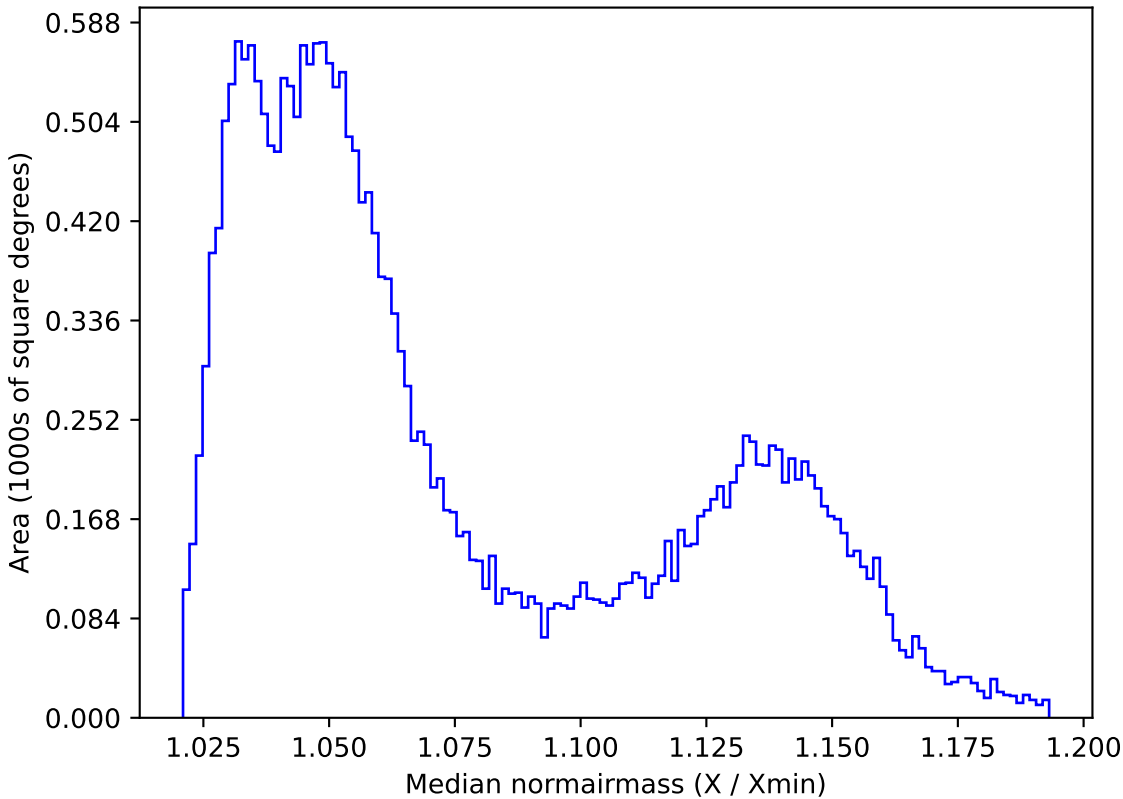
too_10_1v3.4_10yrs All sky all bands: Median normairmass
