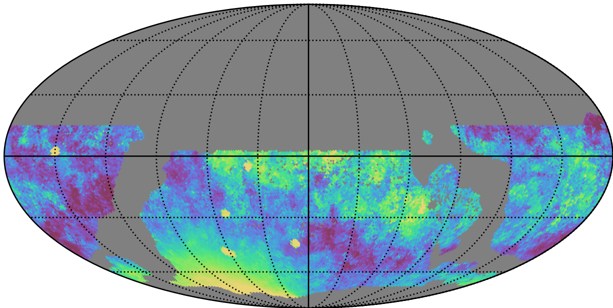
too_10_1v3.4_10yrs WFD z band: Median moonDistance
