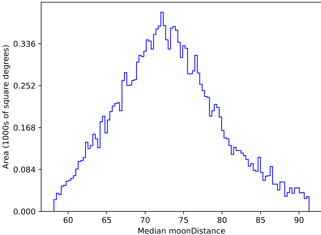
too_10_1v3.4_10yrs WFD z band: Median moonDistance
