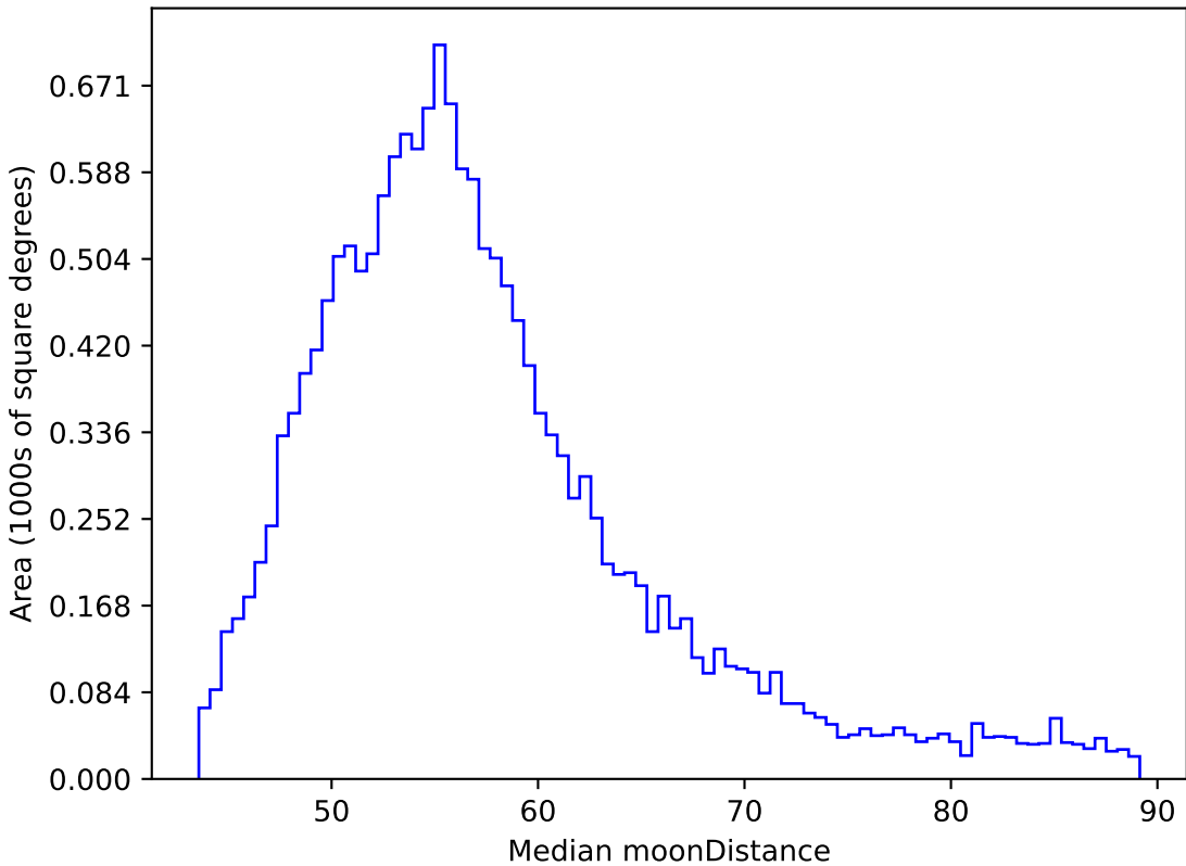
too_10_1v3.4_10yrs WFD y band: Median moonDistance
