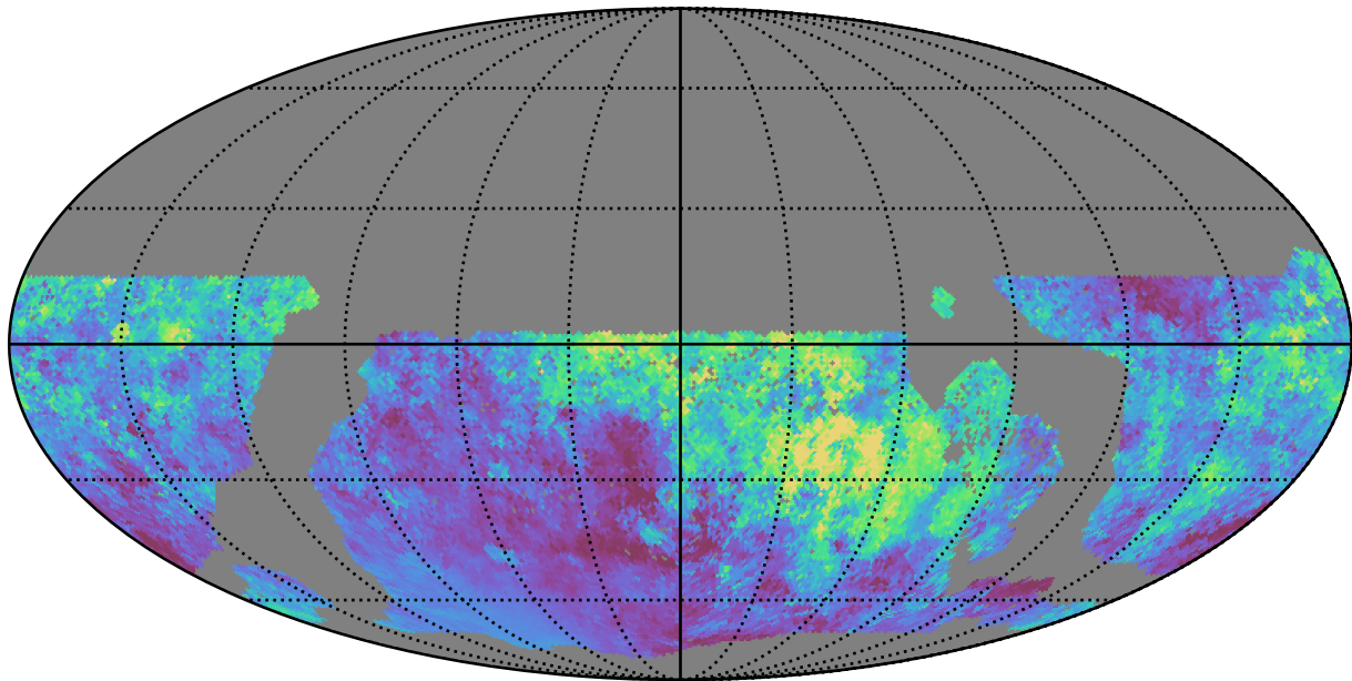
too_10_1v3.4_10yrs WFD i band: Median moonDistance
